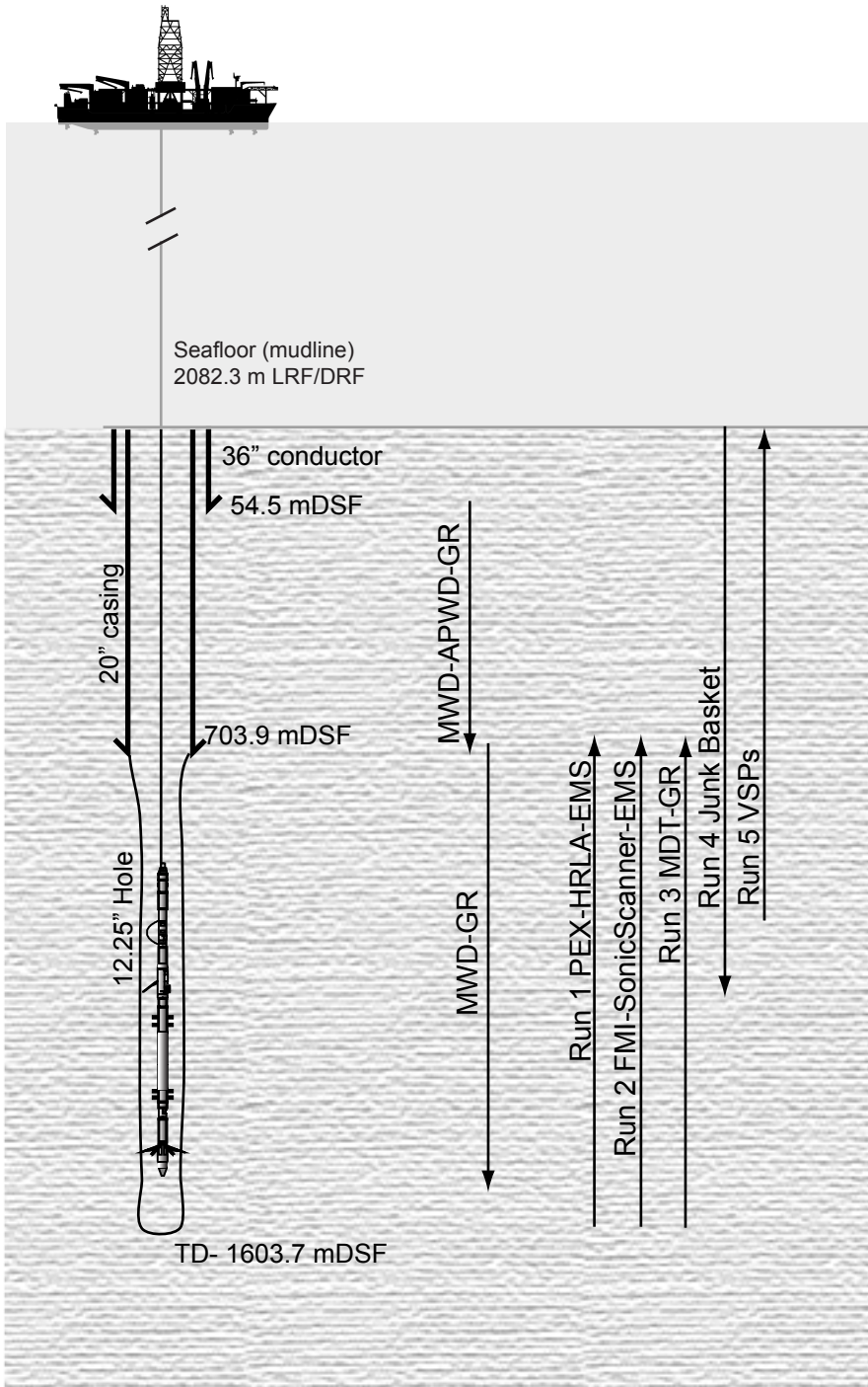
Figure 1. Downhole logging runs at Hole C0009A.
