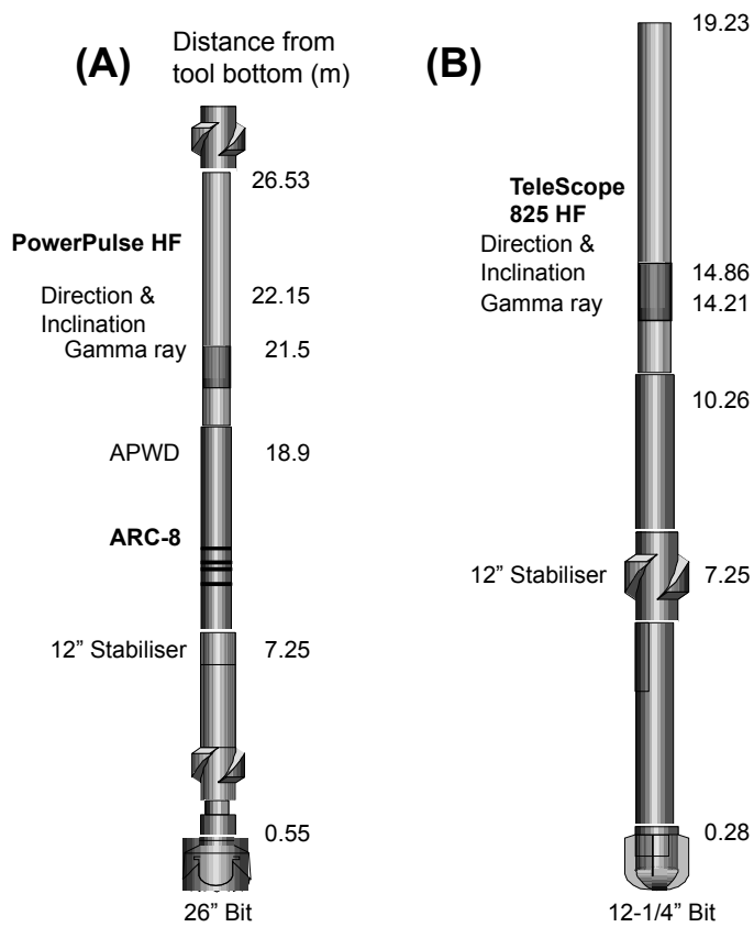
Figure 2. MWD-LWD tool strings used in Hole C0009A. (A) 26" hole bit assembly used between seafloor and 711.8 m LSF, (B) 12 1/4" bit assembly used between 707.7 and 1509.7 m LSF.
