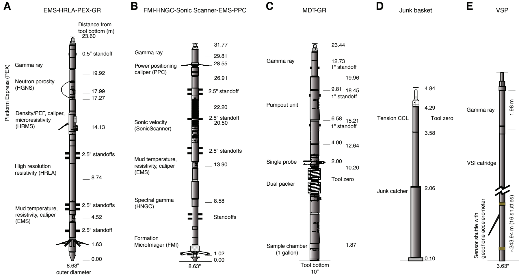
Figure 3. Wireline logging tool strings used in Expedition 319. A. Environmental Measurement Sonde (EMS)–High-Resolution Laterolog Array (HRLA)–Platform Express (PEX)–gamma ray (GR). HGNS = Highly Integrated Gamma Ray Neutron Sonde, PEF = photoelectric effect, HRMS = High-Resolution Mechanical Sonde. B. Formation Microlmager (FMI)-Hostile Natural Gamma Ray Spectrometry Cartridge (HNGC)-Sonic Scanner-EMS-Power Positioning Device and Caliper Tool (PPC). C. Modular Formation Dynamics Tester (MDT)-GR. D. Junk basket. CCL = casing-collar log. E. Walkaway and zero-offset vertical seismic profile (VSP). Each shuttle connected by wireline. VSI = Versatile Seismic Imager.
