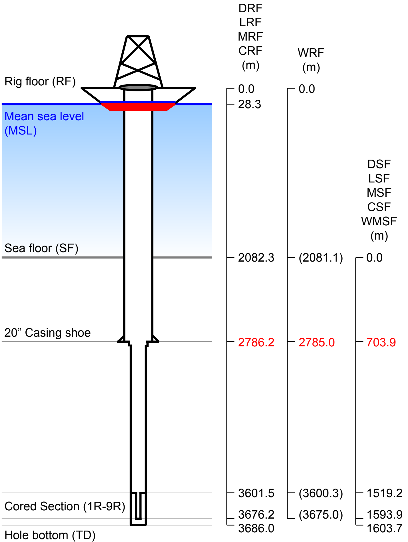
Figure 4. Reference depths and comparison between depth scales at Hole C0009A
