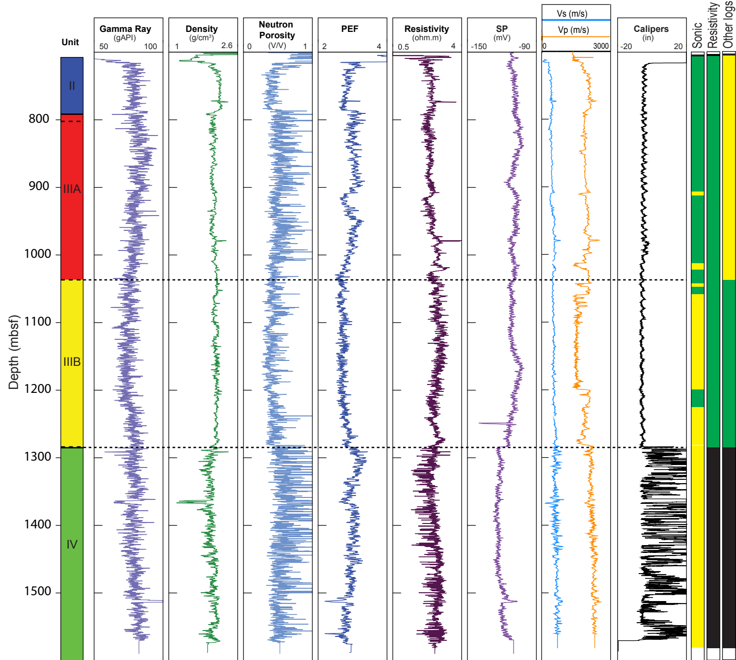
Fig. 5. Wireline logs collected at Hole C0009A and their data quality indicators.
